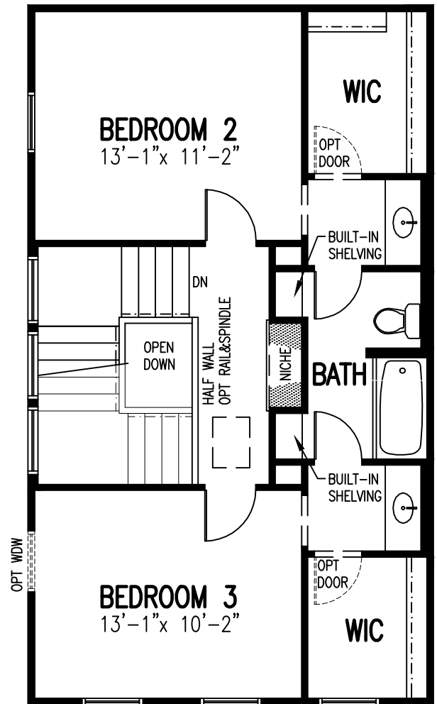
Second Floor Plan with Opt Jack & Jill Bath* Optional
